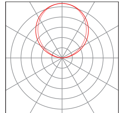
Frosted glass — C0 / C180 cd / 1000 lm - - - C90 / C270
